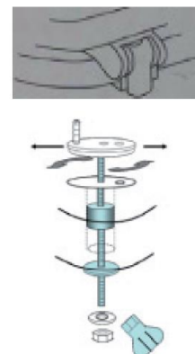
Hinges fixing details
