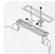
Hinges fixing details
