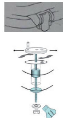
Hinges fixing details
