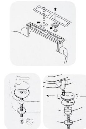
Hinges fixing details
